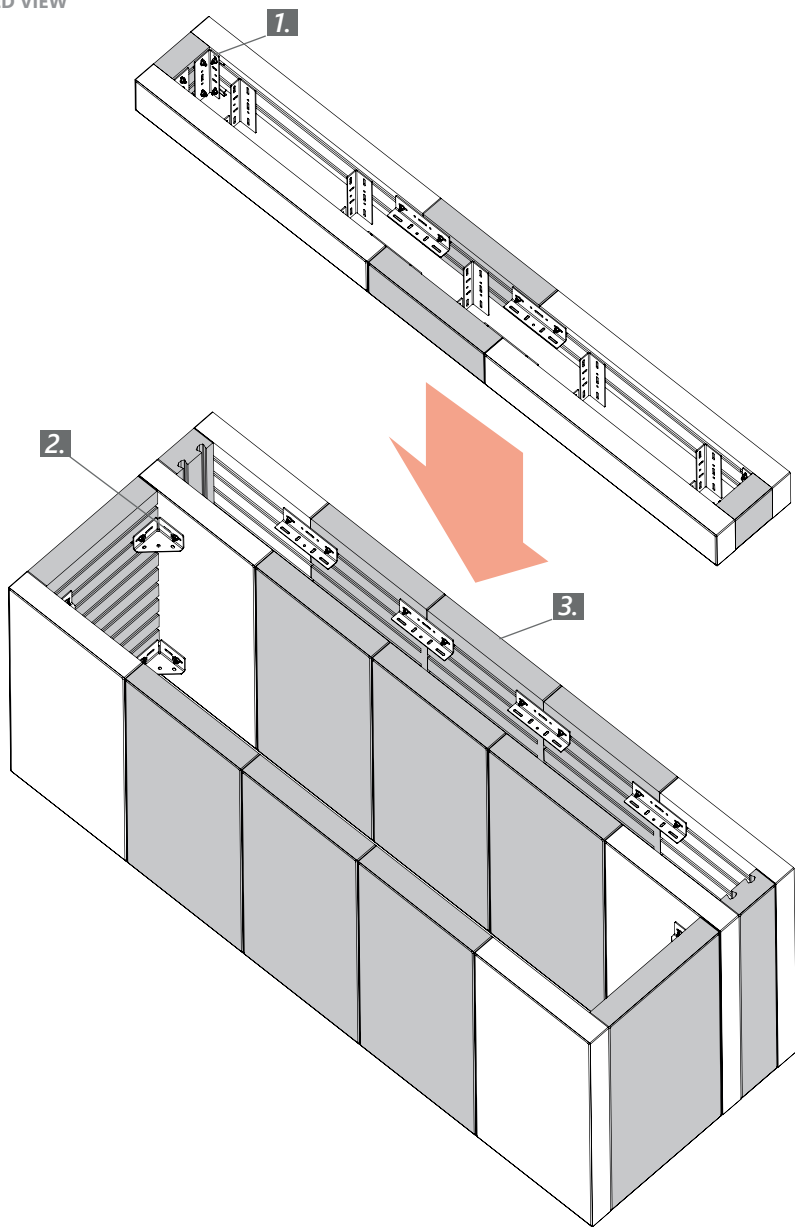
EXPLODED VIEW
