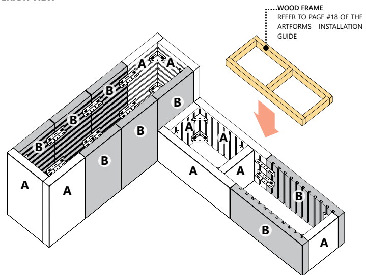
INTERIOR VIEW
