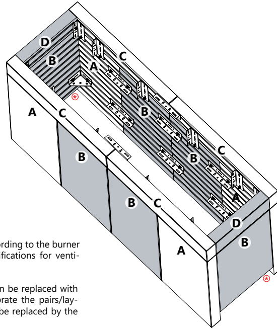
INTERIOR VIEW
